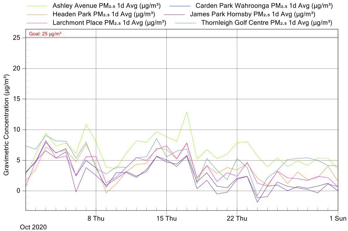
Figure 5: NorthConnex Project Air Monitoring Stations - PM 2.5 1 Day Averages for October 2020
