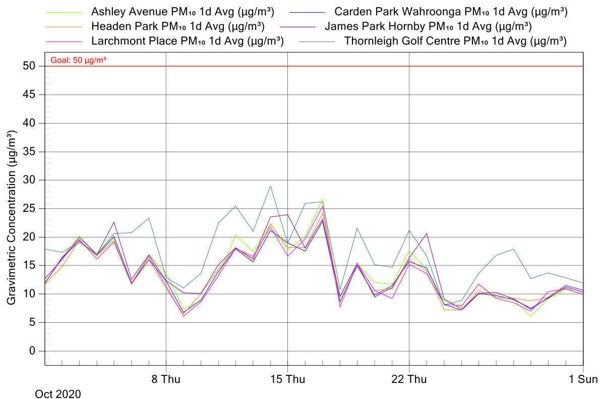
Figure 4: NorthConnex Project Air Monitoring Stations - PM 10 1 Day Averages for October 2020
