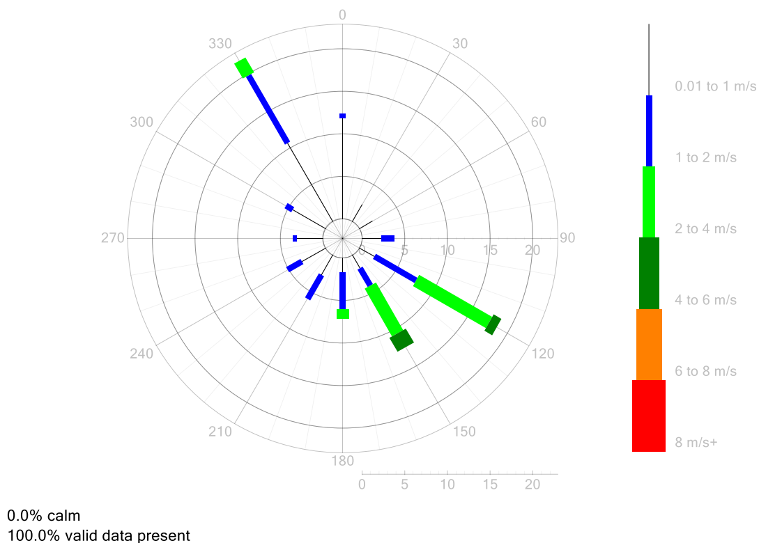
Figure 8: Headen Park – Wind Rose for October 2020
