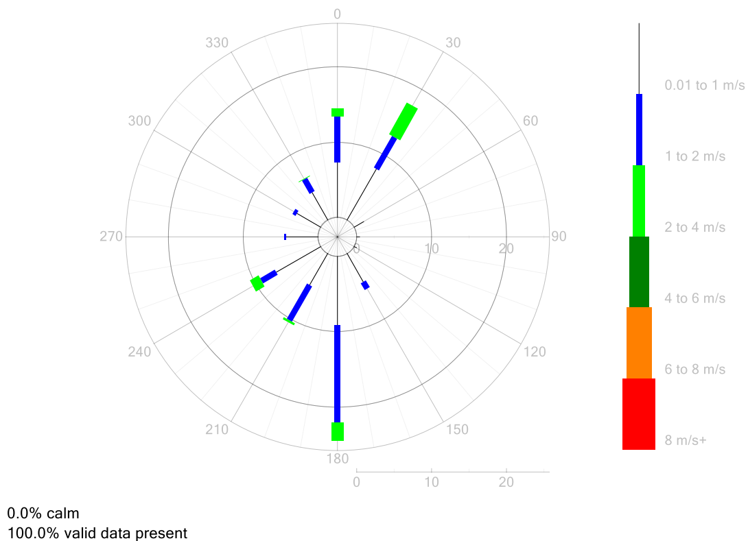
Figure 6: Ashley Avenue – Wind Rose for October 2020
