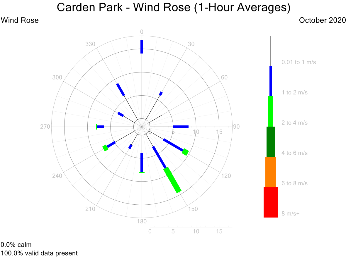
Figure 7: Carden Park – Wind Rose for October 2020
