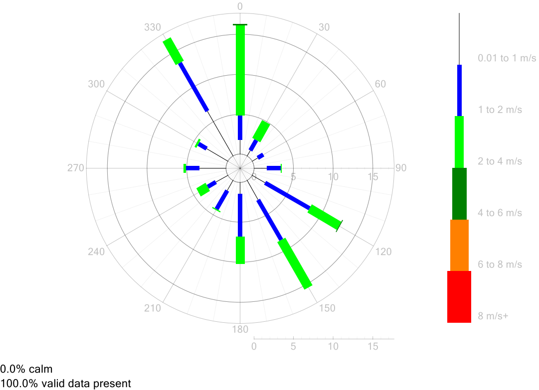
Figure 11: Thornleigh Golf Centre – Wind Rose for October 2020
