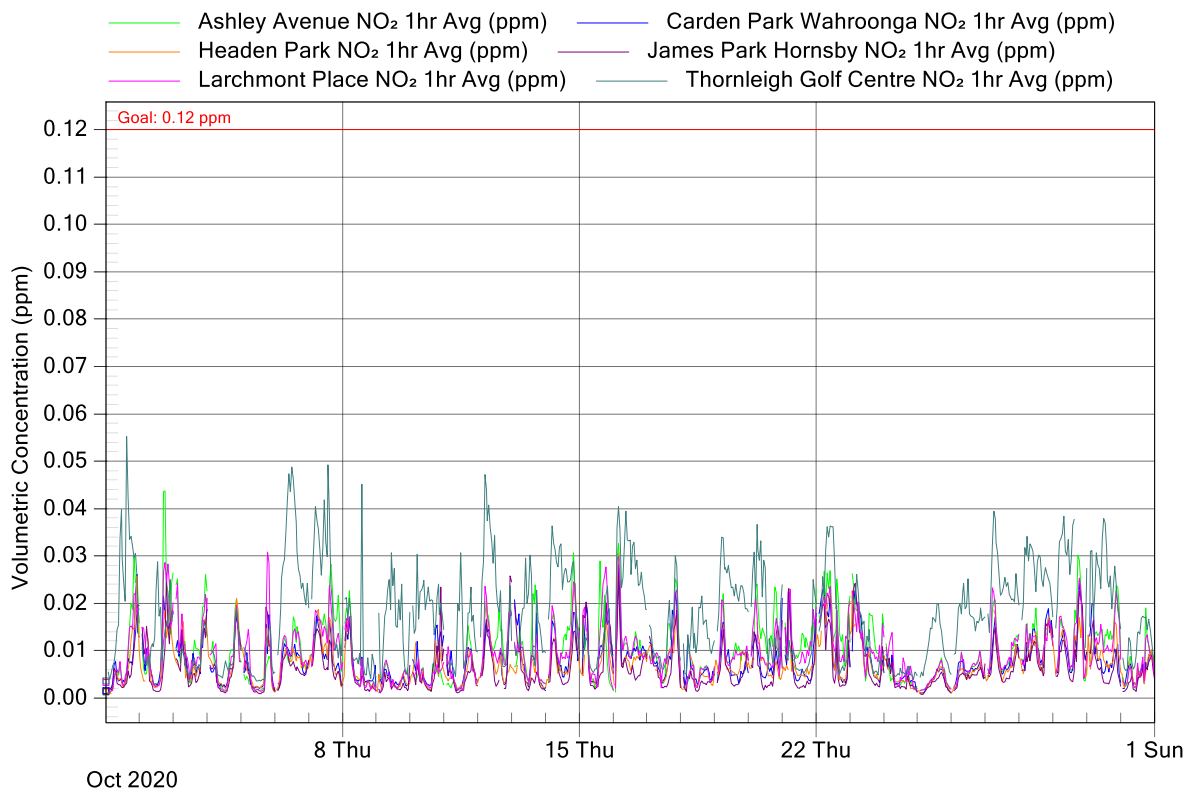
Figure 3: NorthConnex Project Air Monitoring Stations - NO 2 1 Hour Averages for October 2020
