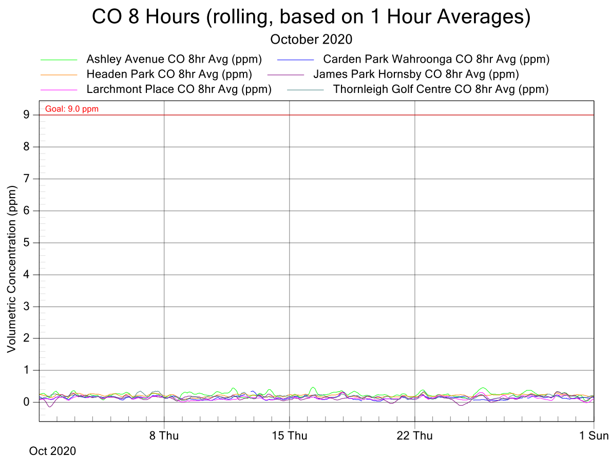
Figure 2: NorthConnex Project Air Monitoring Stations - CO 8 Hours Rolling Averages for October 2020
