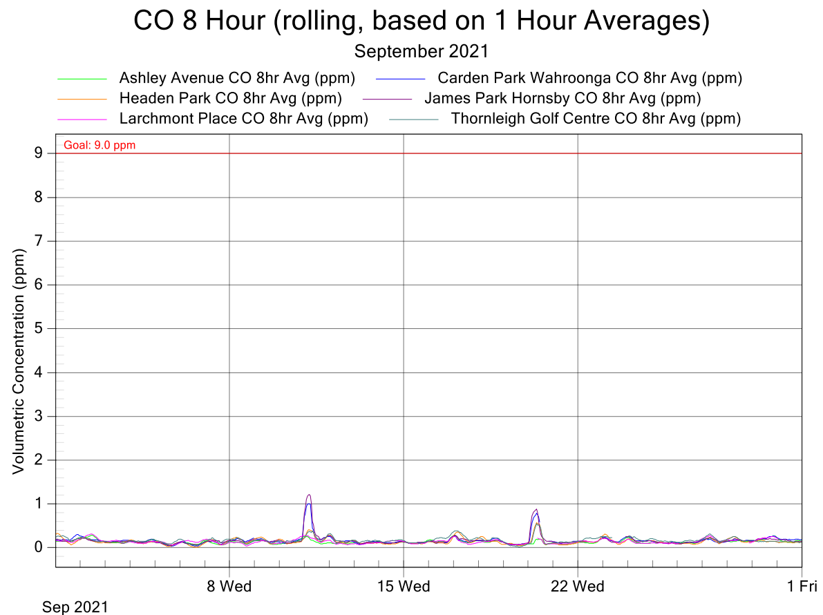
Figure 2: NorthConnex Project Air Monitoring Stations - CO 8 Hour Rolling Averages for September 2021
