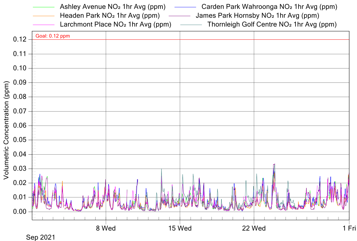
Figure 3: NorthConnex Project Air Monitoring Stations - NO 2 1 Hour Averages for September 2021
