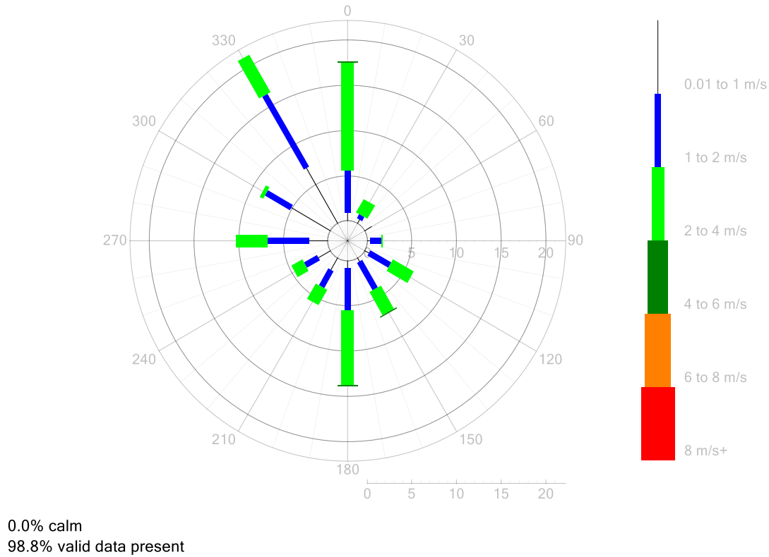
Figure 11: Thornleigh Golf Centre – Wind Rose for September 2021
