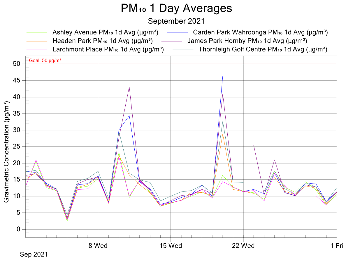
Figure 4: NorthConnex Project Air Monitoring Stations - PM 10 1 Day Averages for September 2021
