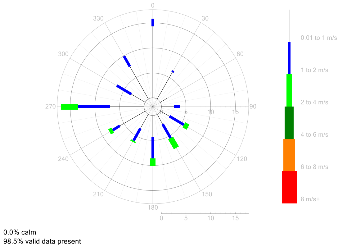
Figure 7: Carden Park – Wind Rose for September 2021
