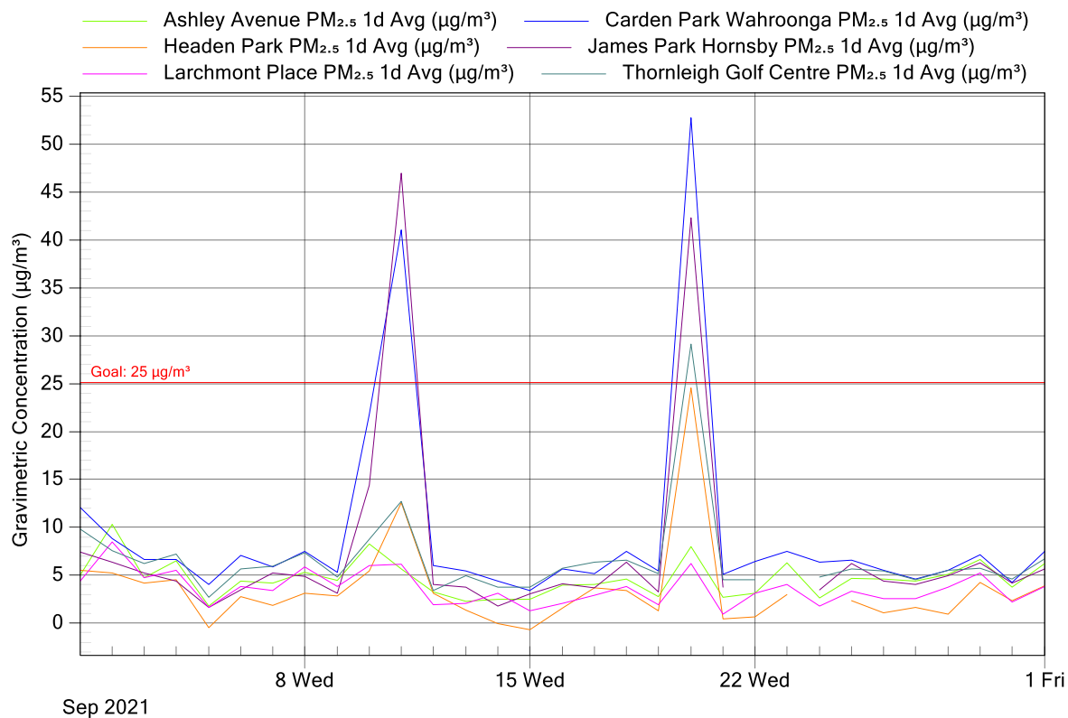
Figure 5: NorthConnex Project Air Monitoring Stations - PM 2.5 1 Day Averages for September 2021
