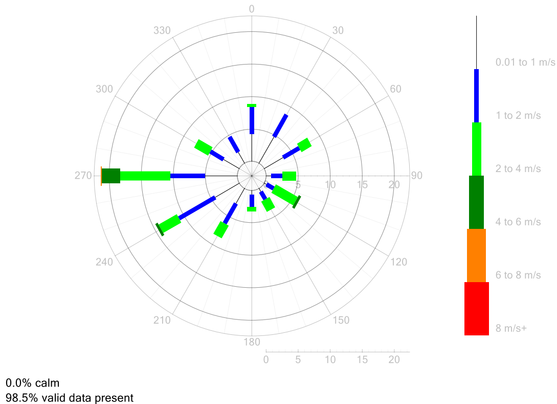
Figure 9: James Park Hornsby – Wind Rose for September 2021
