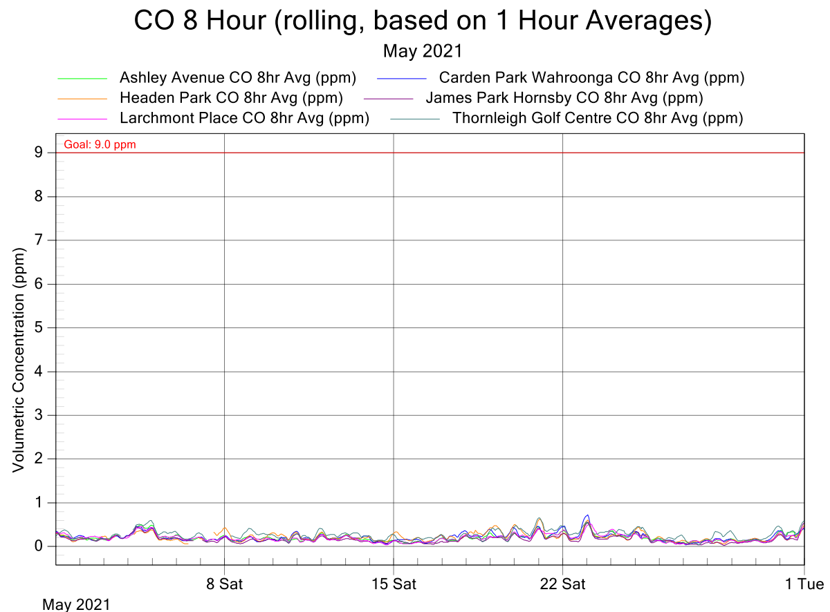
Figure 2: NorthConnex Project Air Monitoring Stations - CO 8 Hour Rolling Averages for May 2021
