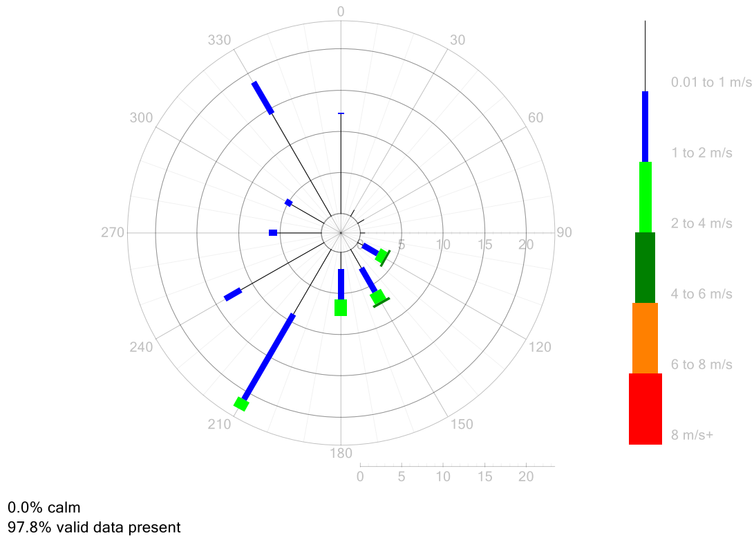
Figure 8: Headen Park – Wind Rose for May 2021
