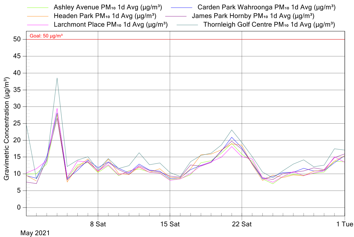
Figure 4: NorthConnex Project Air Monitoring Stations - PM 10 1 Day Averages for May 2021
