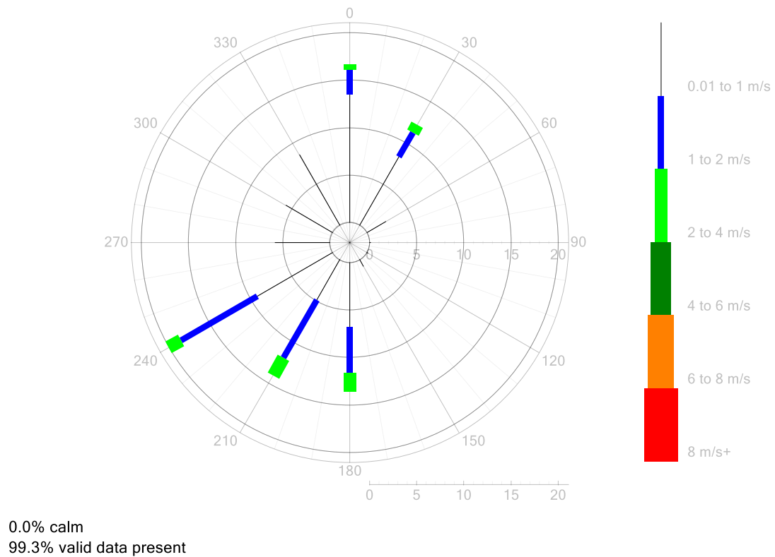
Figure 6: Ashley Avenue – Wind Rose for May 2021
