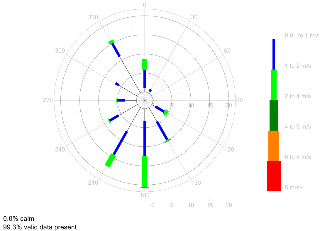
Figure 11: Thornleigh Golf Centre – Wind Rose for May 2021
