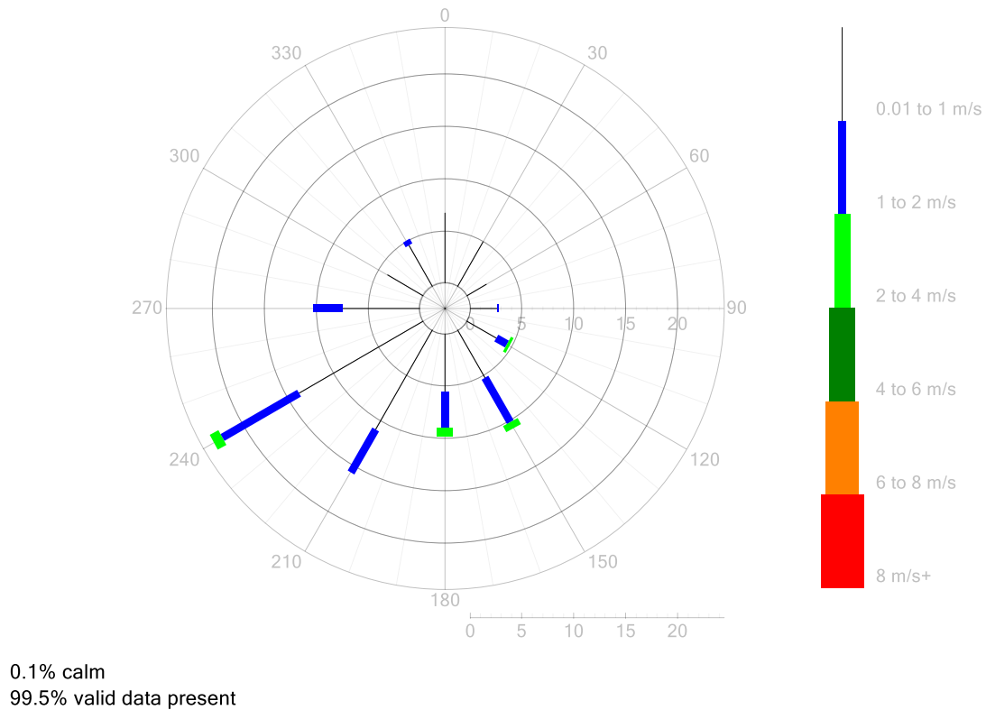
Figure 7: Carden Park – Wind Rose for May 2021
