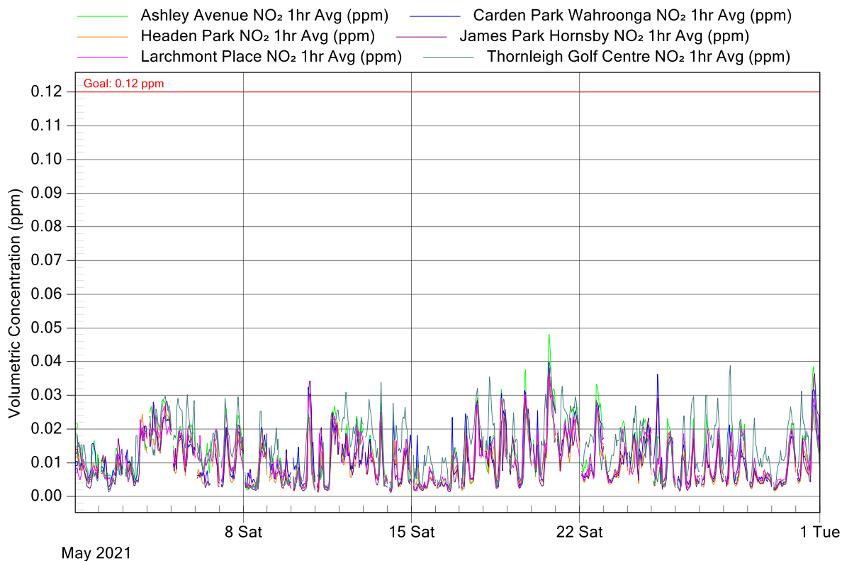
Figure 3: NorthConnex Project Air Monitoring Stations - NO 2 1 Hour Averages for May 2021
