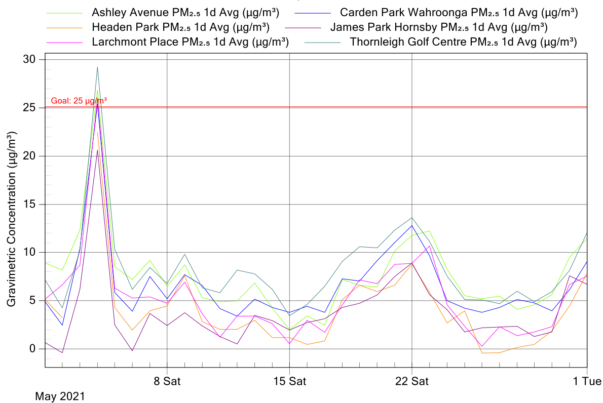
Figure 5: NorthConnex Project Air Monitoring Stations - PM 2.5 1 Day Averages for May 2021
