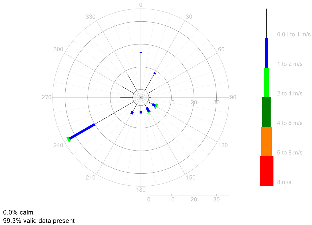
Figure 10: Larchmont Place – Wind Rose for May 2021
