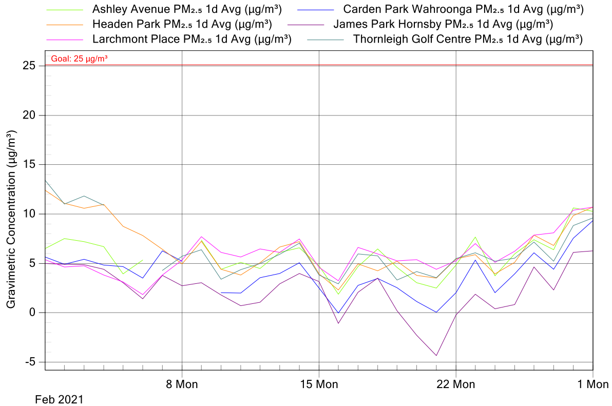
Figure 5: NorthConnex Project Air Monitoring Stations - PM 2.5 1 Day Averages for February 2021
