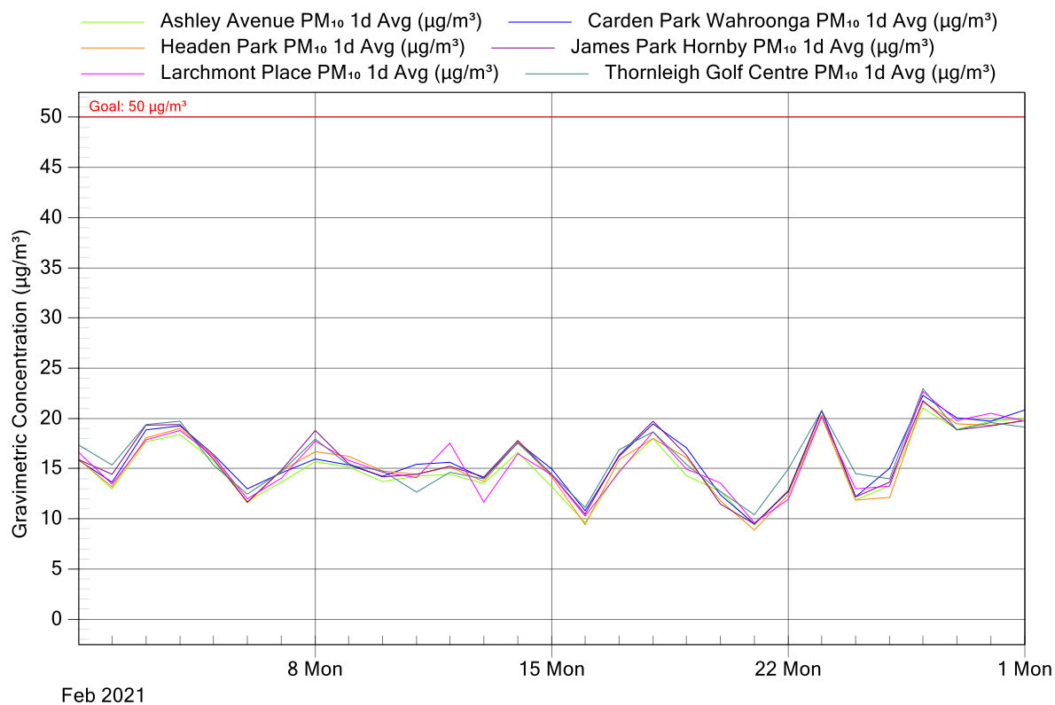
Figure 4: NorthConnex Project Air Monitoring Stations - PM 10 1 Day Averages for February 2021
