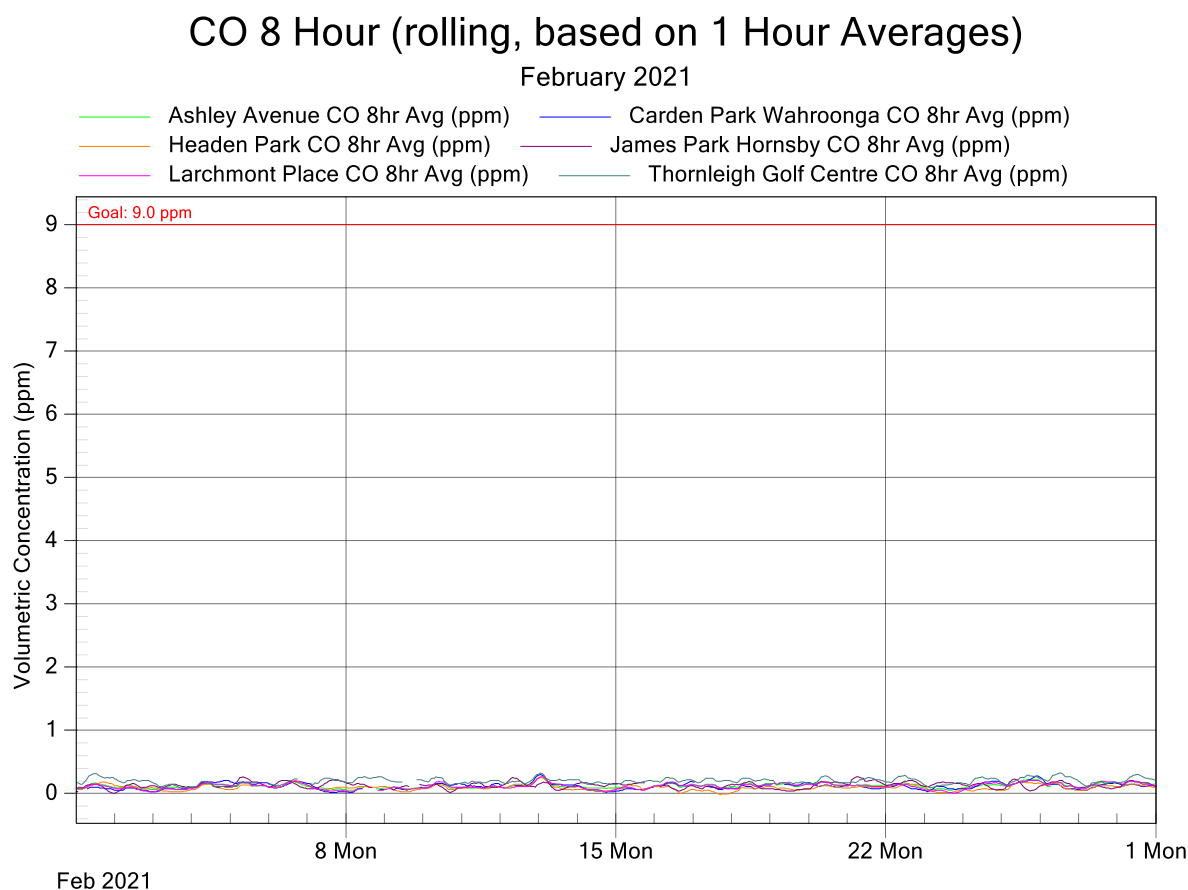
Figure 2: NorthConnex Project Air Monitoring Stations - CO 8 Hour Rolling Averages for February 2021
