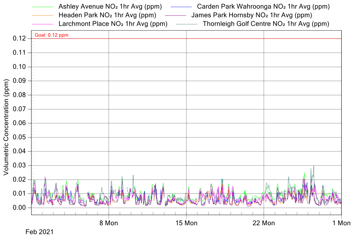
Figure 3: NorthConnex Project Air Monitoring Stations - NO 2 1 Hour Averages for February 2021
