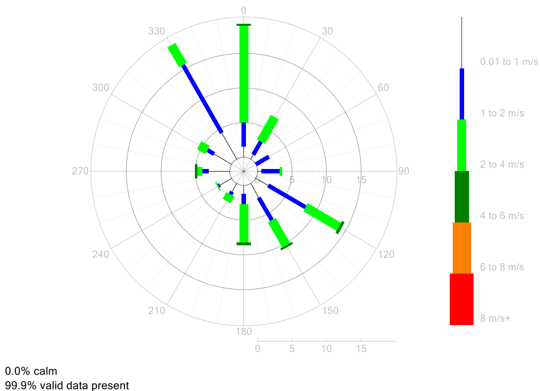
Figure 11: Thornleigh Golf Centre – Wind Rose for November 2020
