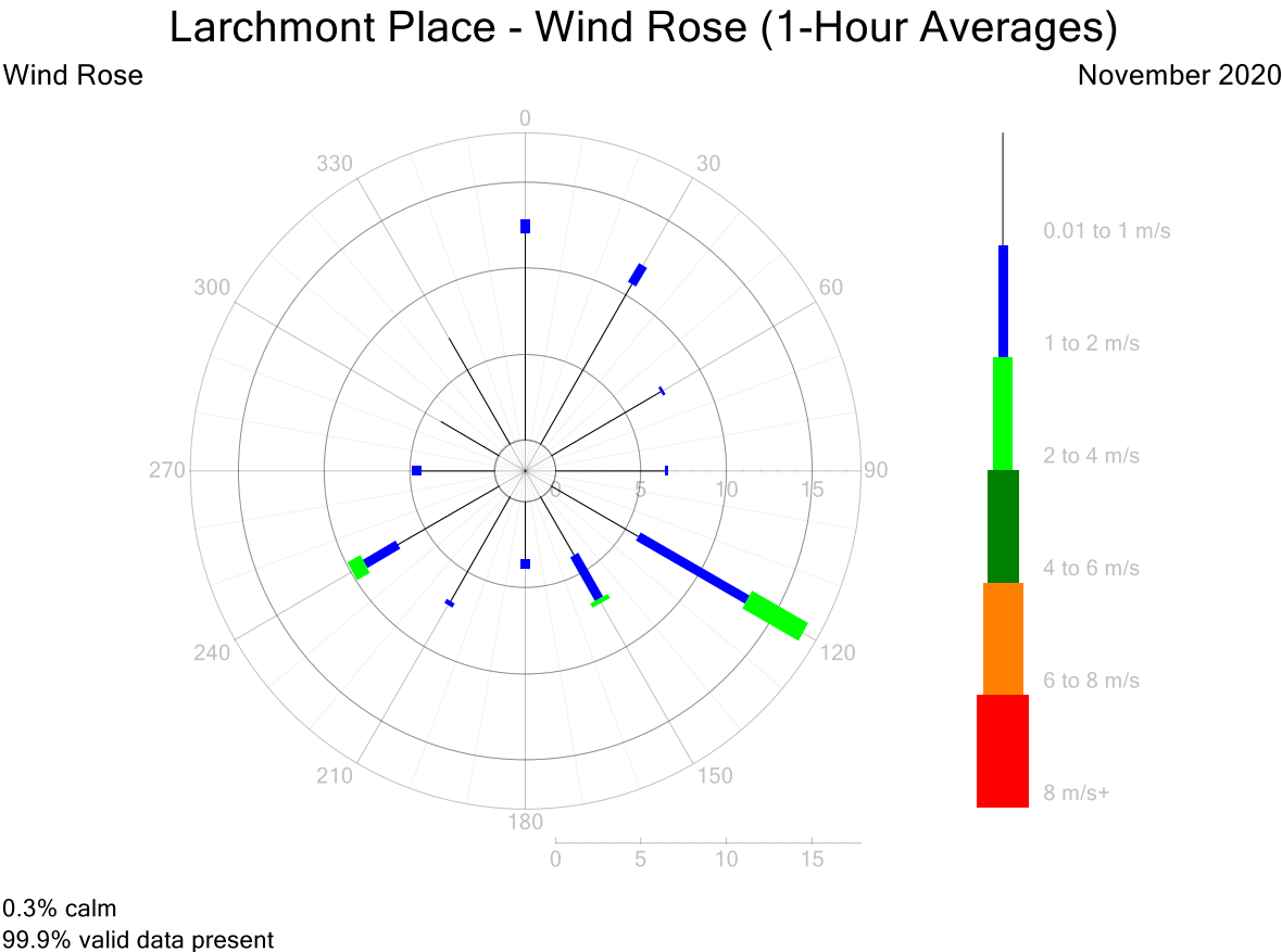
Figure 10: Larchmont Place – Wind Rose for November 2020
