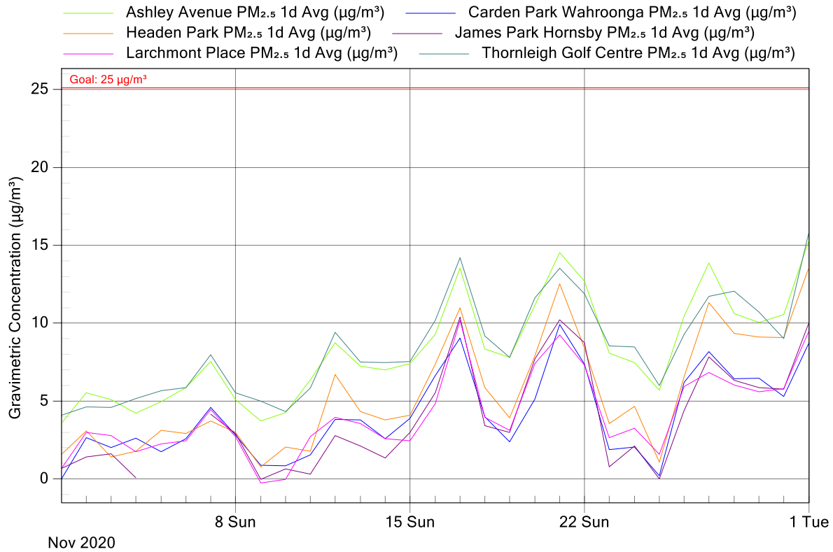
Figure 5: NorthConnex Project Air Monitoring Stations - PM 2.5 1 Day Averages for November 2020
