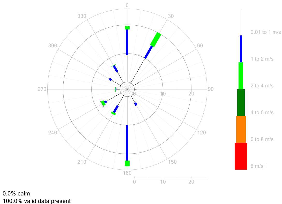
Figure 6: Ashley Avenue – Wind Rose for November 2020
