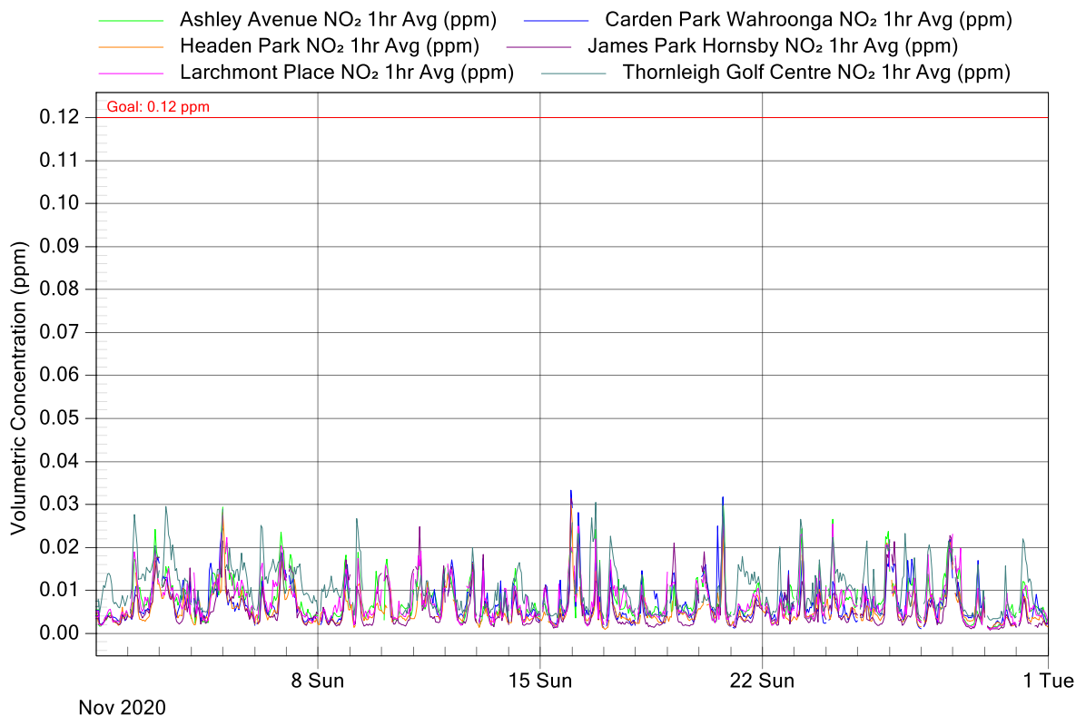
Figure 3: NorthConnex Project Air Monitoring Stations - NO 2 1 Hour Averages for November 2020
