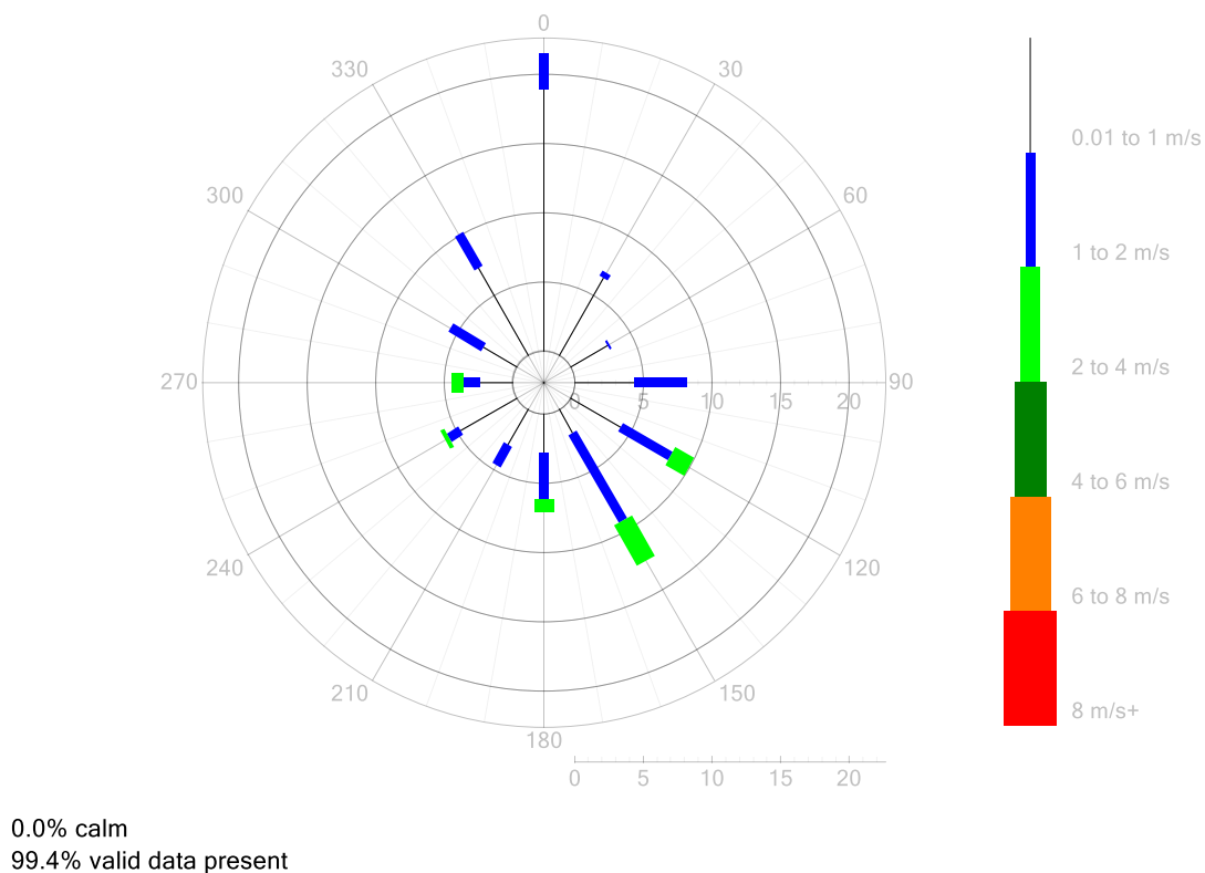
Figure 7: Carden Park – Wind Rose for November 2020
