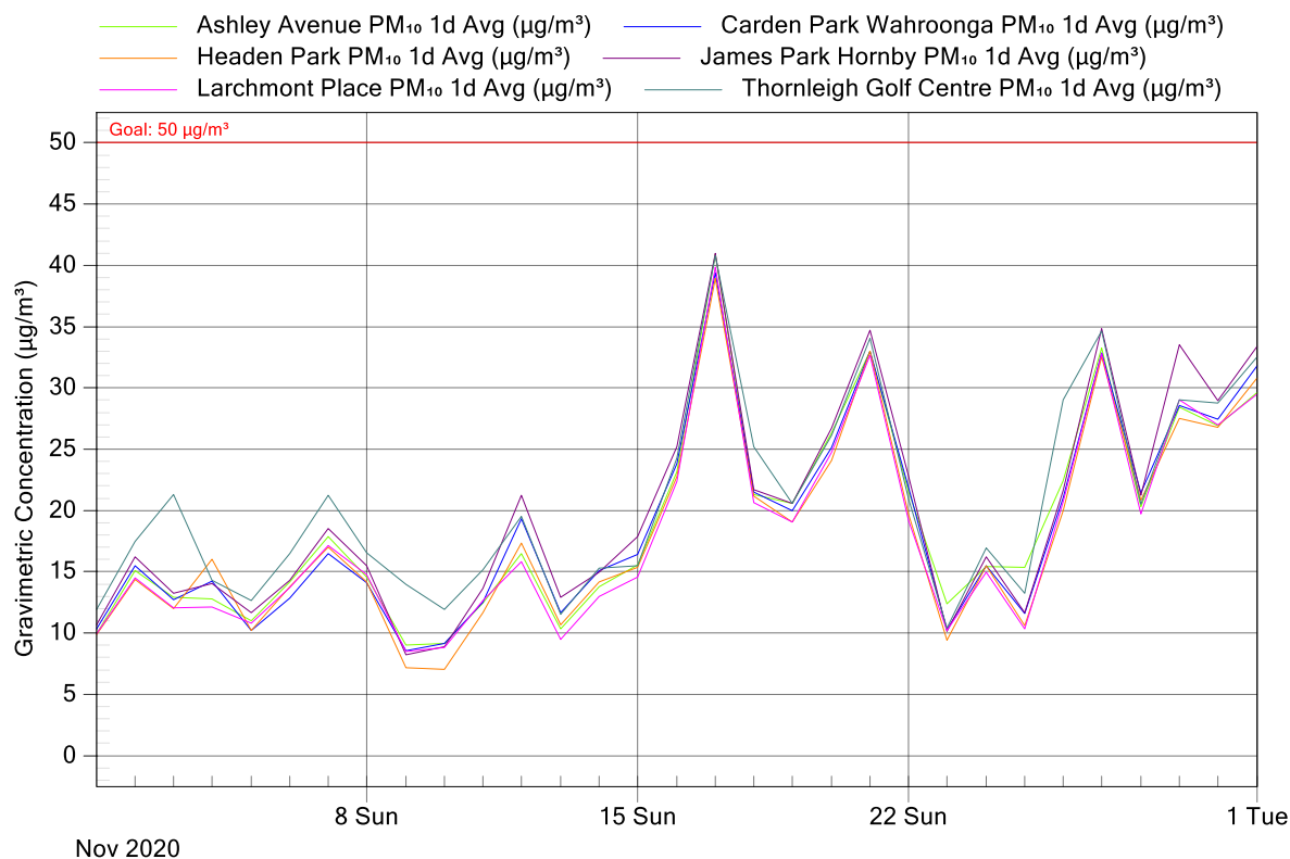
Figure 4: NorthConnex Project Air Monitoring Stations - PM 10 1 Day Averages for November 2020
